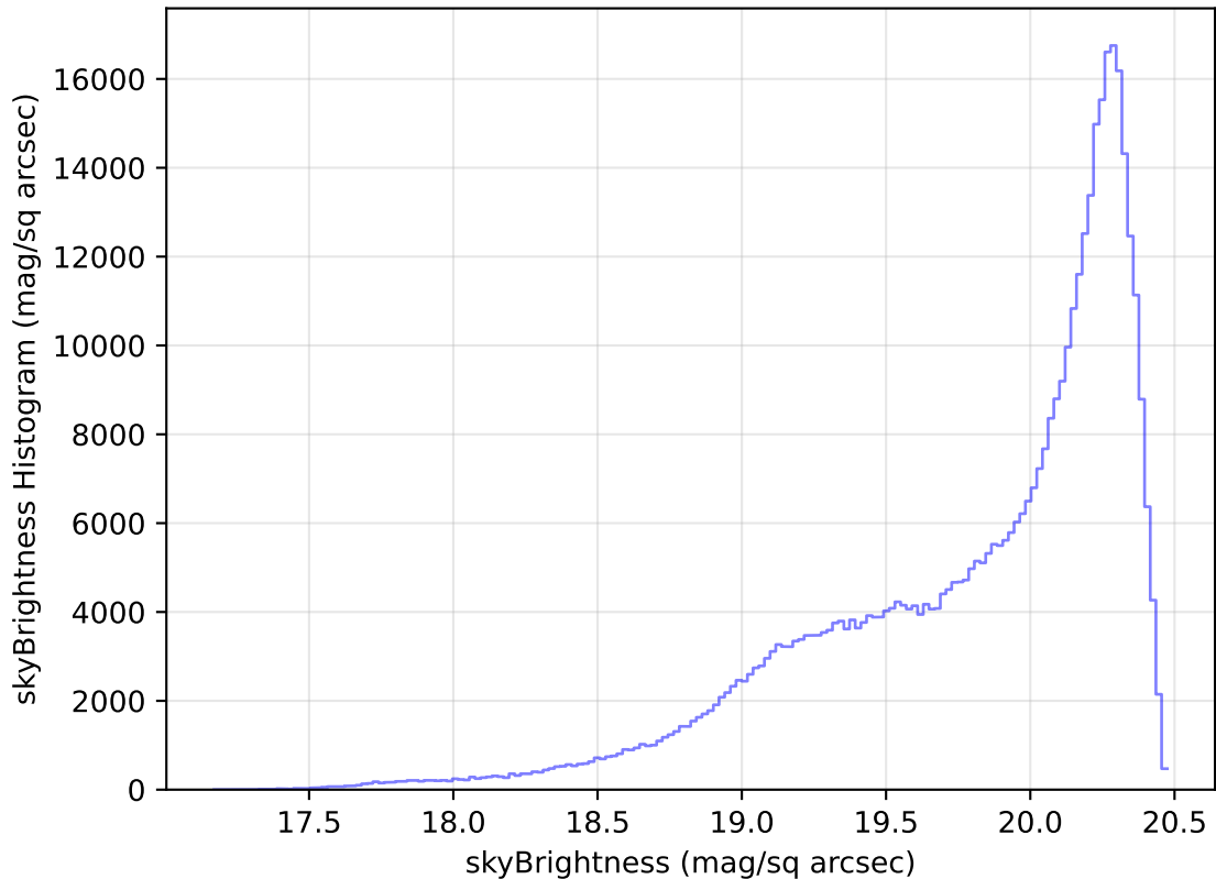
ddf_loaded_fl2_v3.4_10yrs WFD i band: skyBrightness Histogram
