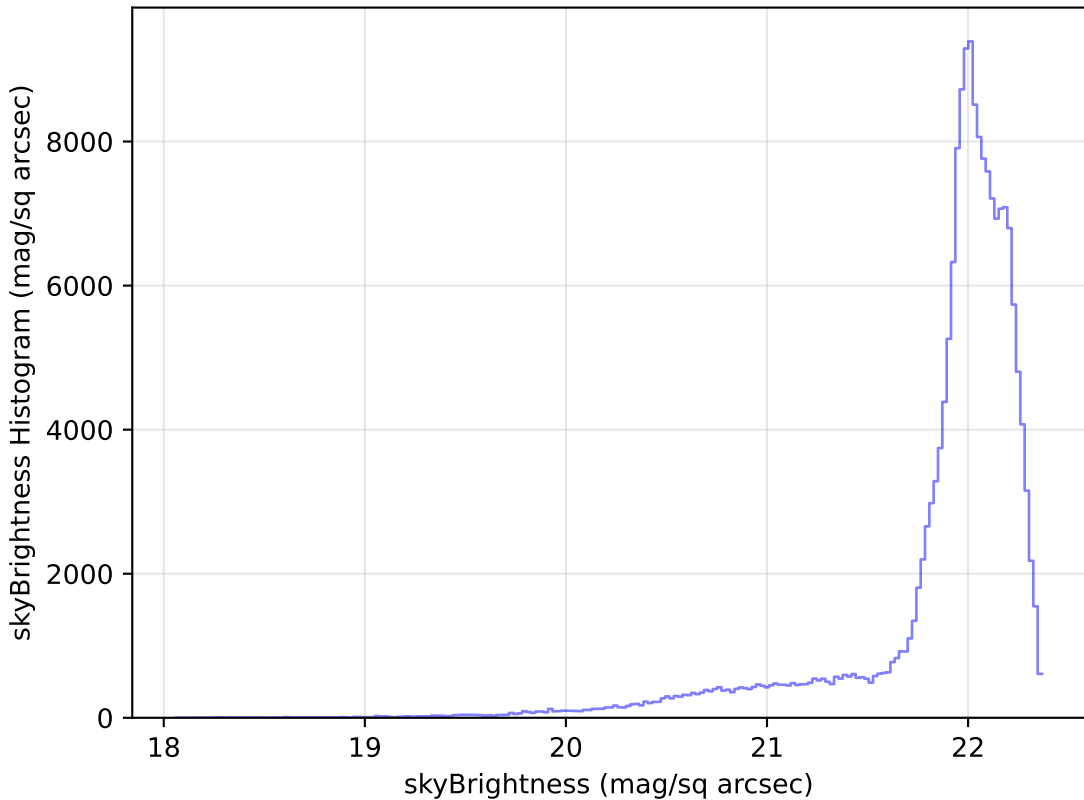
ddf_loaded_fl2_v3.4_10yrs WFD g band: skyBrightness Histogram
