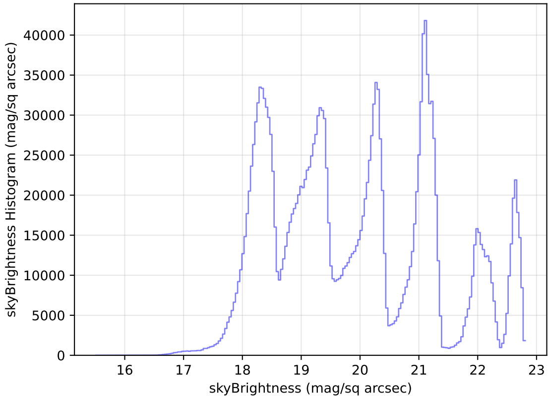
ddf_loaded_fl2_v3.4_10yrs WFD all bands: skyBrightness Histogram
