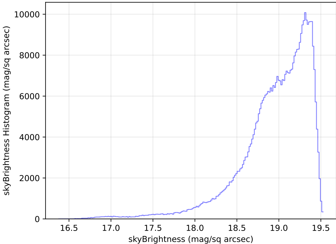
ddf_loaded_fl2_v3.4_10yrs All sky z band: skyBrightness Histogram
