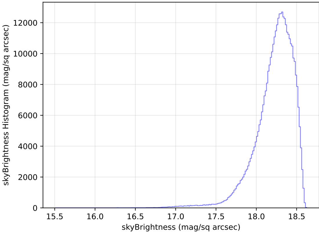
ddf_loaded_fl2_v3.4_10yrs All sky y band: skyBrightness Histogram
