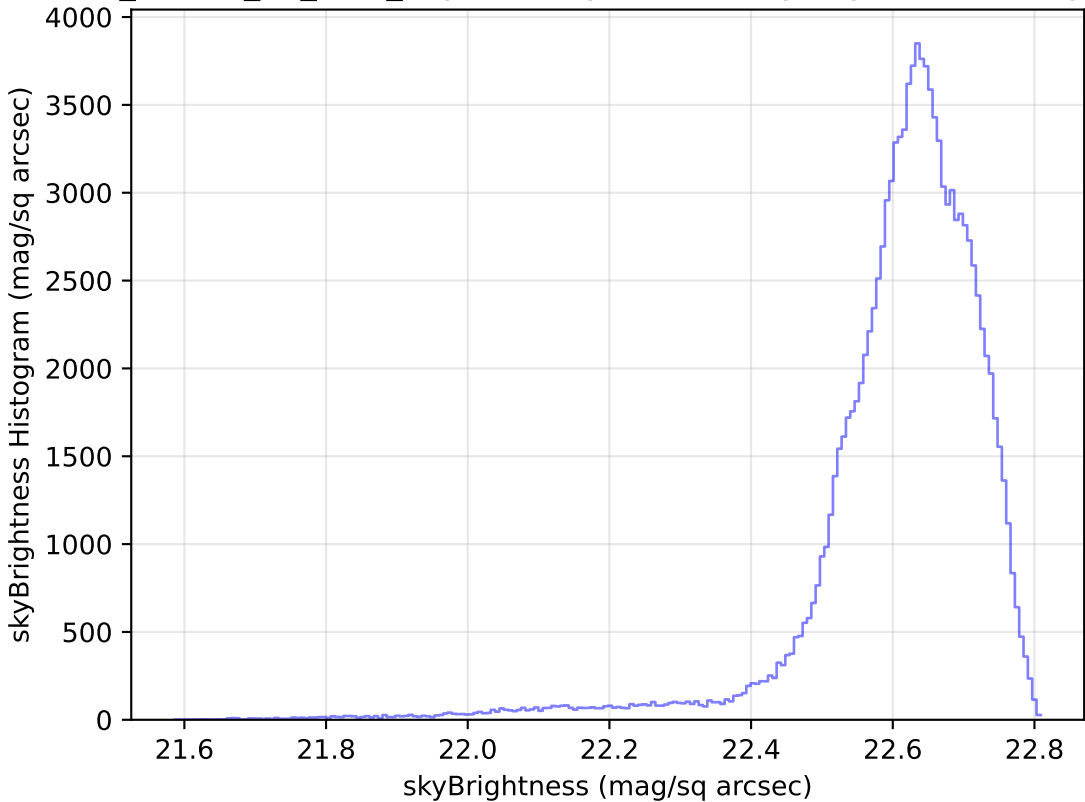
ddf_loaded_fl2_v3.4_10yrs All sky u band: skyBrightness Histogram
