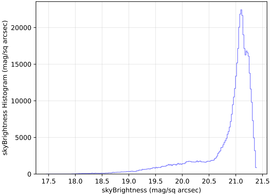
ddf_loaded_fl2_v3.4_10yrs All sky r band: skyBrightness Histogram
