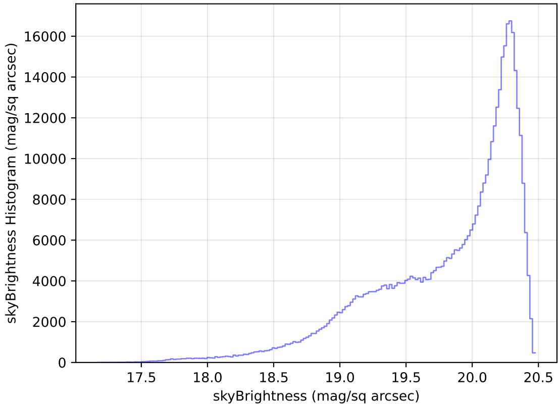
ddf_loaded_fl2_v3.4_10yrs All sky i band: skyBrightness Histogram
