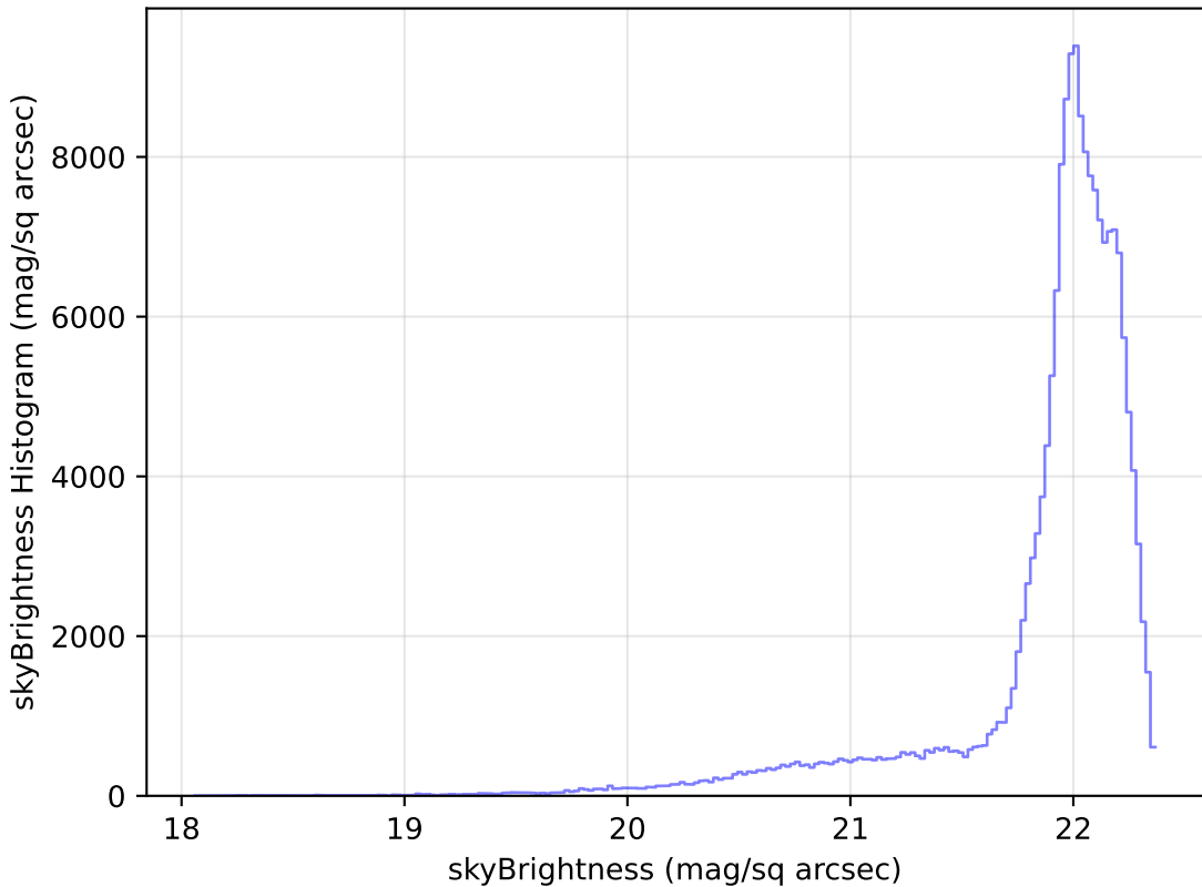
ddf_loaded_fl2_v3.4_10yrs All sky g band: skyBrightness Histogram
