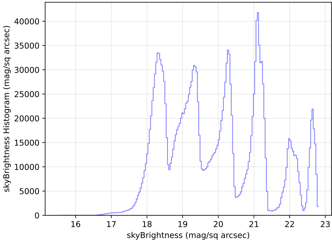
ddf_loaded_fl2_v3.4_10yrs All sky all bands: skyBrightness Histogram
