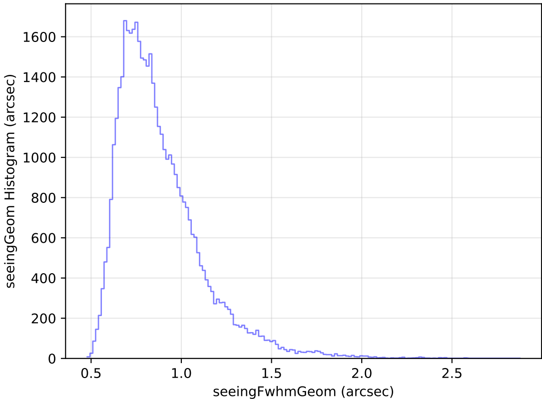
ddf_loaded_fl2_v3.4_10yrs Yr 1 z band: seeingGeom Histogram
