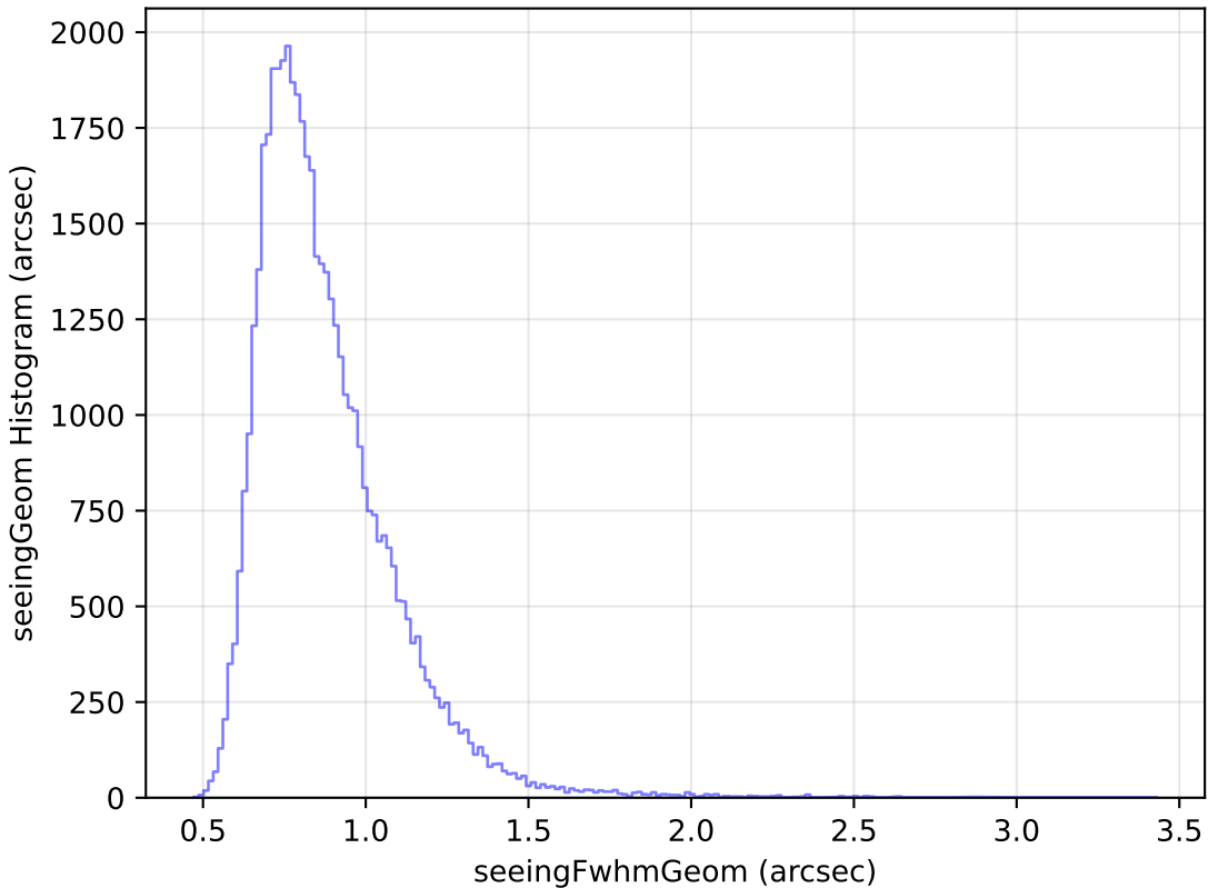
ddf_loaded_fl2_v3.4_10yrs Yr 1 y band: seeingGeom Histogram
