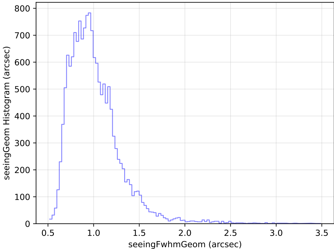
ddf_loaded_fl2_v3.4_10yrs Yr 1 u band: seeingGeom Histogram
