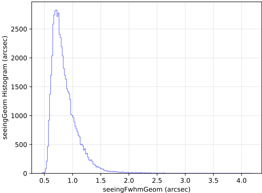
ddf_loaded_fl2_v3.4_10yrs Yr 1 i band: seeingGeom Histogram
