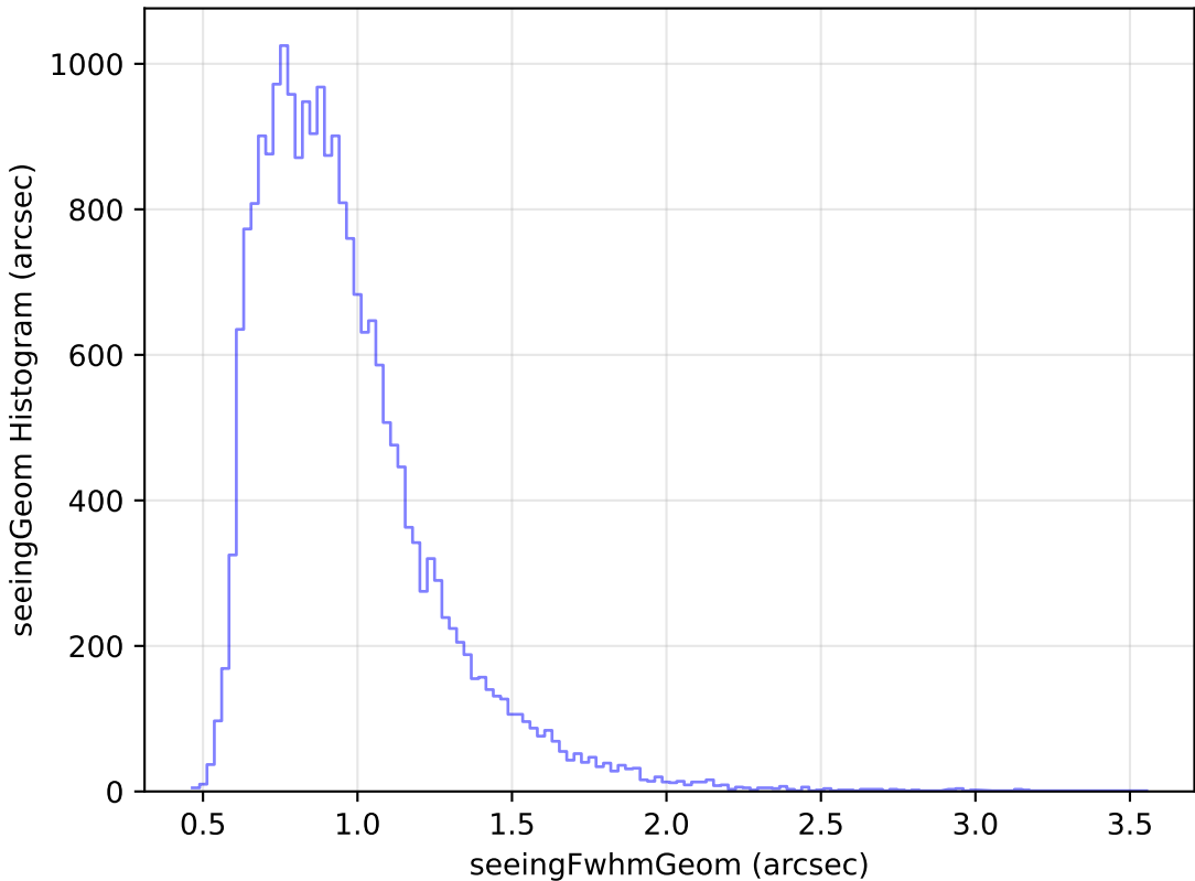
ddf_loaded_fl2_v3.4_10yrs Yr 1 g band: seeingGeom Histogram
