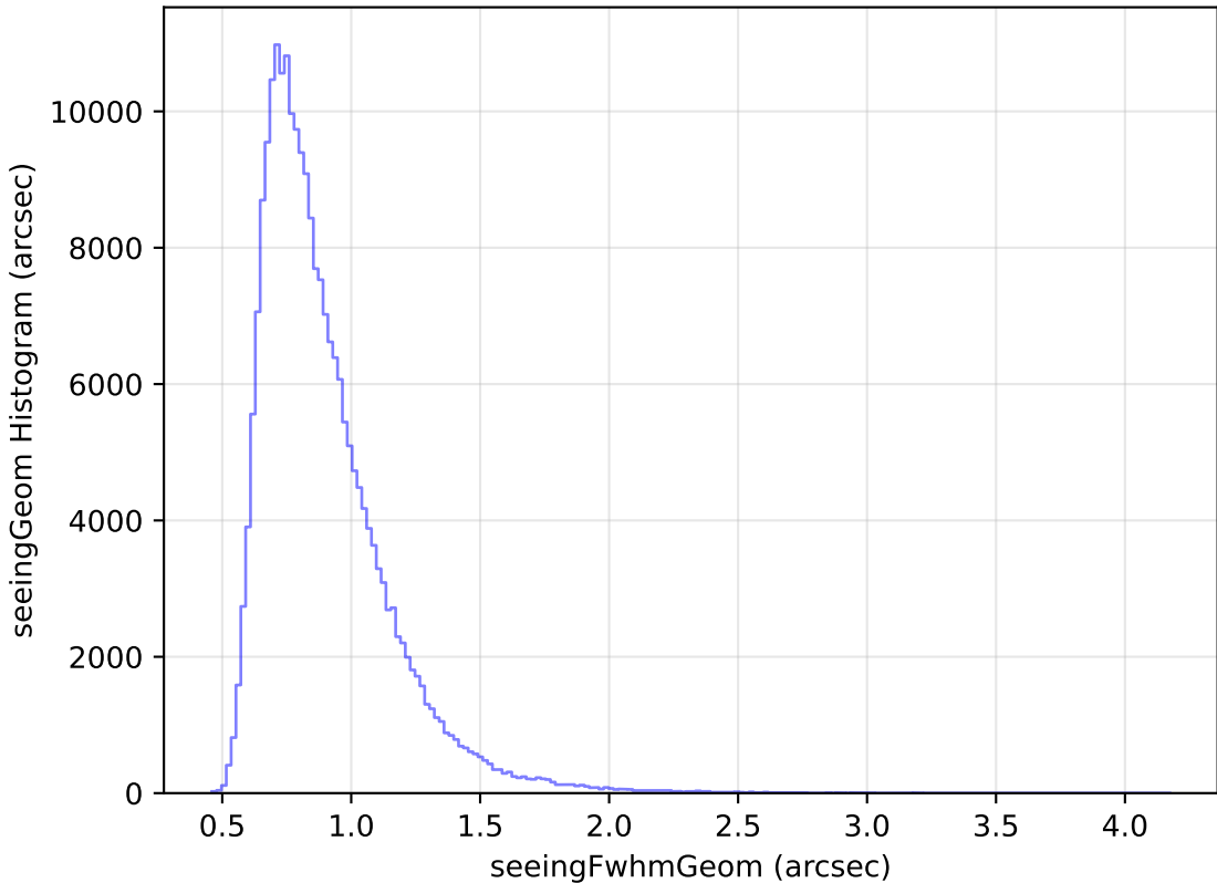
ddf_loaded_fl2_v3.4_10yrs Yr 1 all bands: seeingGeom Histogram
