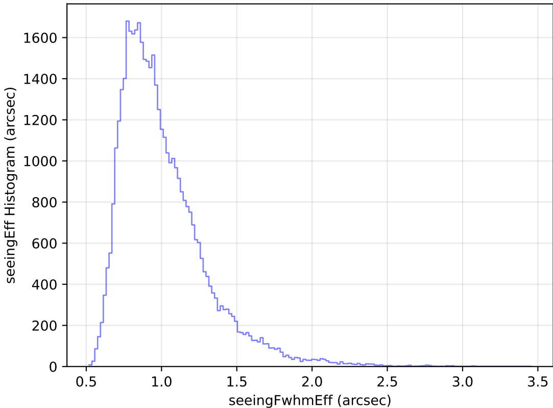
ddf_loaded_fl2_v3.4_10yrs Yr 1 z band: seeingEff Histogram
