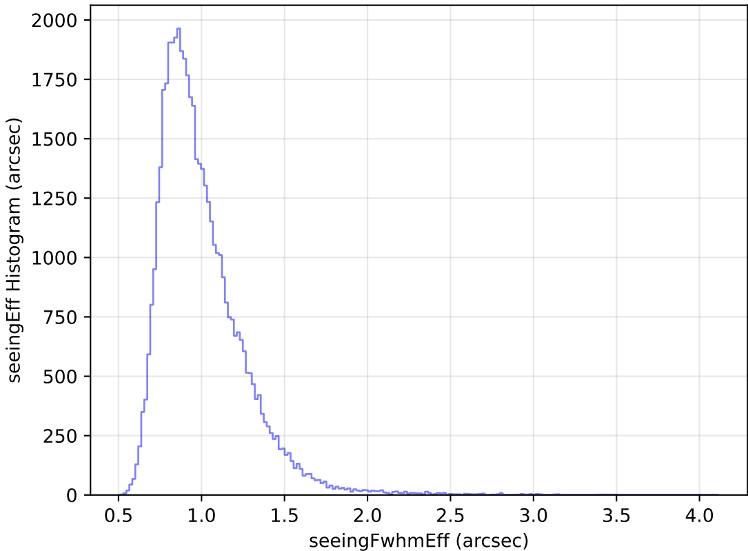
ddf_loaded_fl2_v3.4_10yrs Yr 1 y band: seeingEff Histogram
