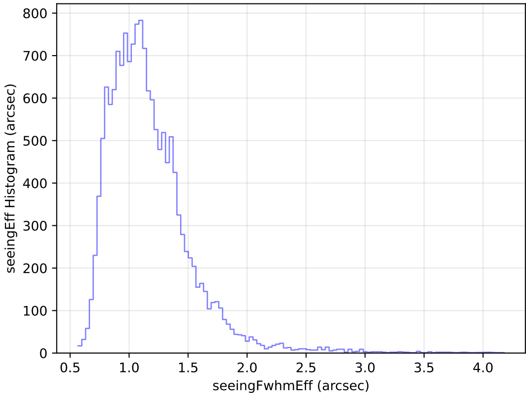
ddf_loaded_fl2_v3.4_10yrs Yr 1 u band: seeingEff Histogram
