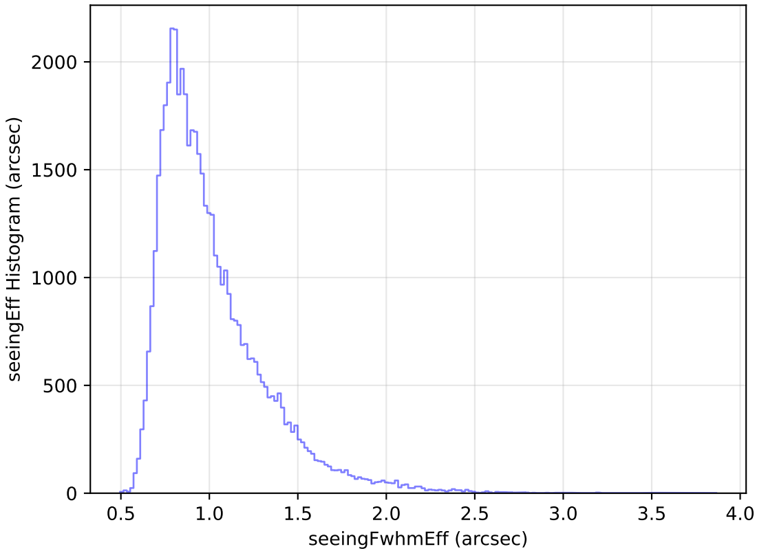
ddf_loaded_fl2_v3.4_10yrs Yr 1 r band: seeingEff Histogram
