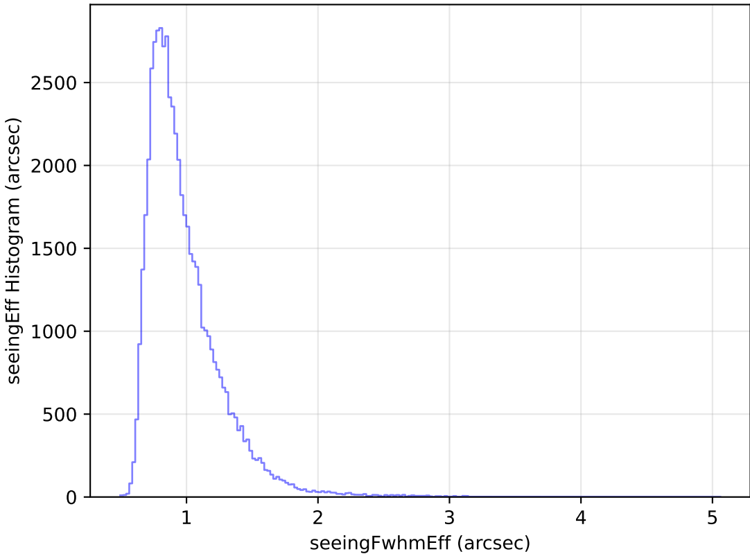
ddf_loaded_fl2_v3.4_10yrs Yr 1 i band: seeingEff Histogram
