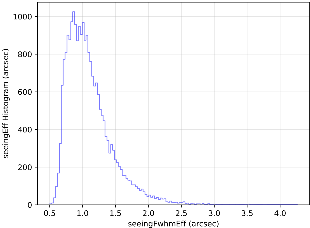
ddf_loaded_fl2_v3.4_10yrs Yr 1 g band: seeingEff Histogram
