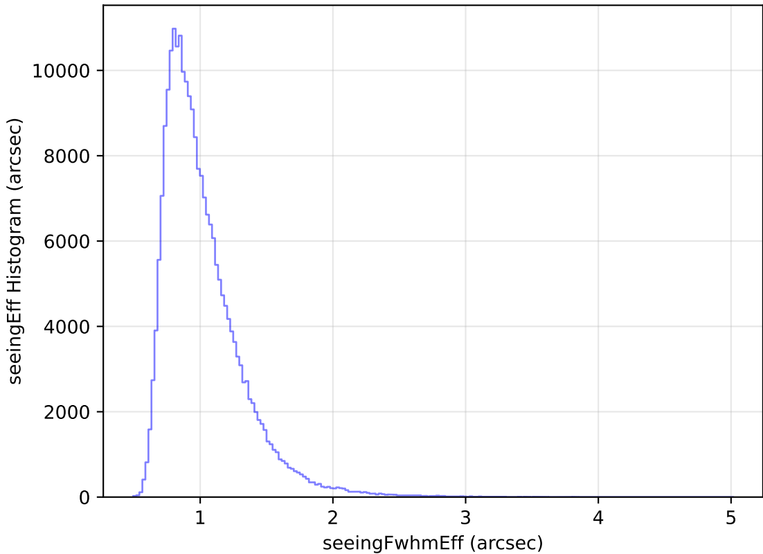
ddf_loaded_fl2_v3.4_10yrs Yr 1 all bands: seeingEff Histogram
