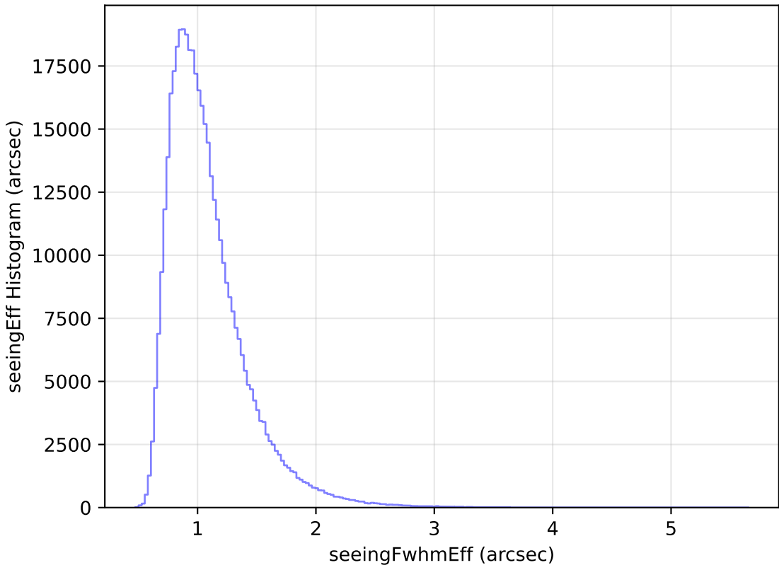
ddf_loaded_fl2_v3.4_10yrs WFD z band: seeingEff Histogram
