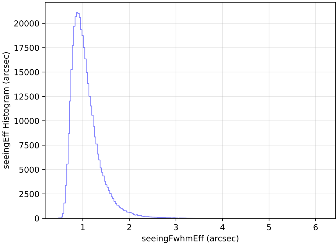
ddf_loaded_fl2_v3.4_10yrs WFD y band: seeingEff Histogram
