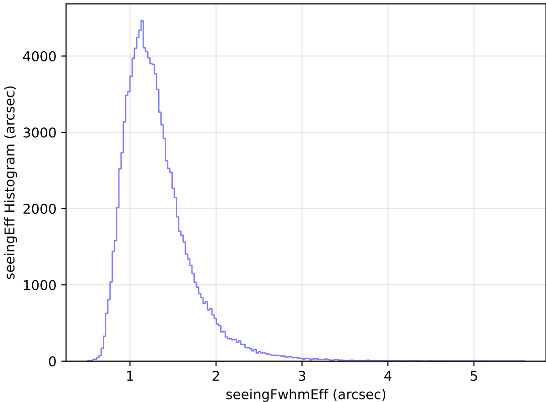
ddf_loaded_fl2_v3.4_10yrs WFD u band: seeingEff Histogram
