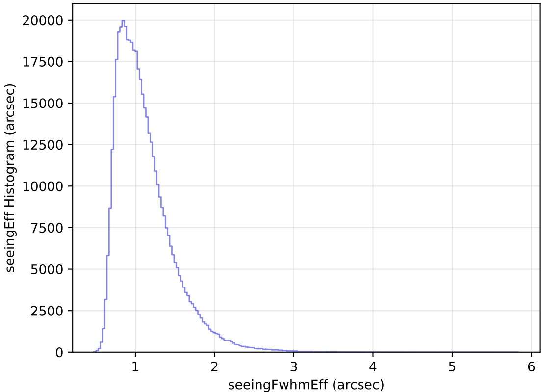
ddf_loaded_fl2_v3.4_10yrs WFD r band: seeingEff Histogram
