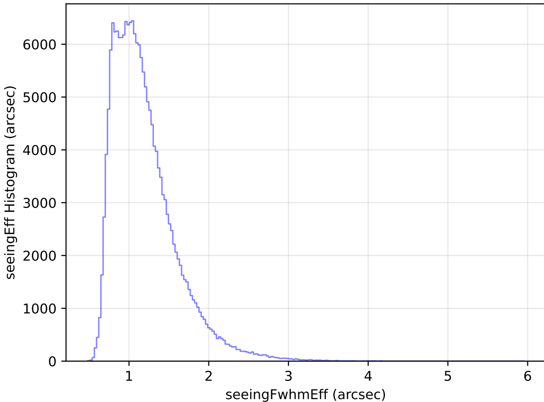
ddf_loaded_fl2_v3.4_10yrs WFD g band: seeingEff Histogram
