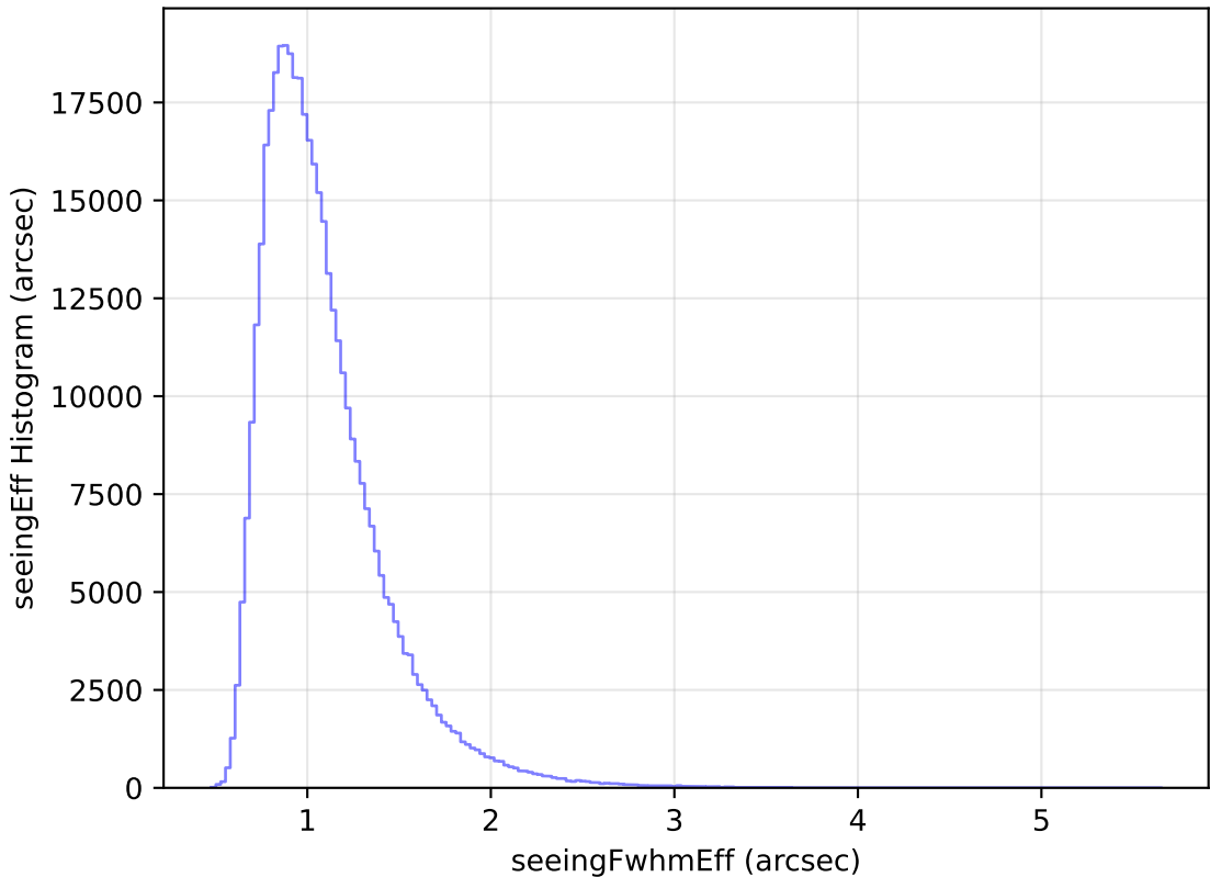
ddf_loaded_fl2_v3.4_10yrs All sky z band: seeingEff Histogram
