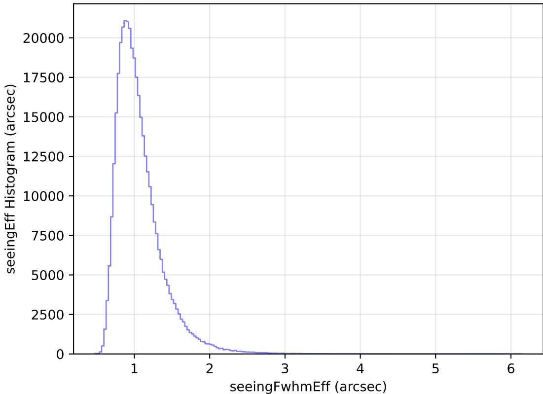
ddf_loaded_fl2_v3.4_10yrs All sky y band: seeingEff Histogram
