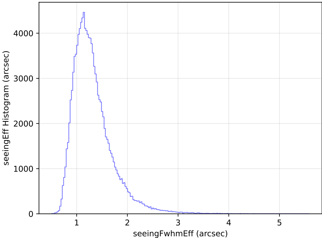
ddf_loaded_fl2_v3.4_10yrs All sky u band: seeingEff Histogram
