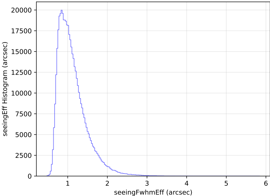
ddf_loaded_fl2_v3.4_10yrs All sky r band: seeingEff Histogram
