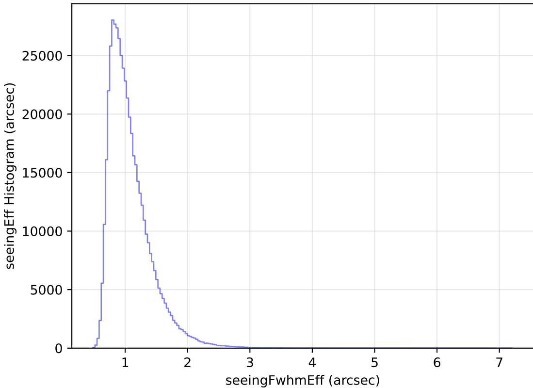
ddf_loaded_fl2_v3.4_10yrs All sky i band: seeingEff Histogram
