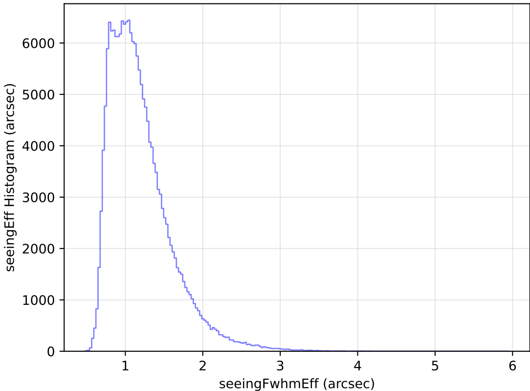
ddf_loaded_fl2_v3.4_10yrs All sky g band: seeingEff Histogram
