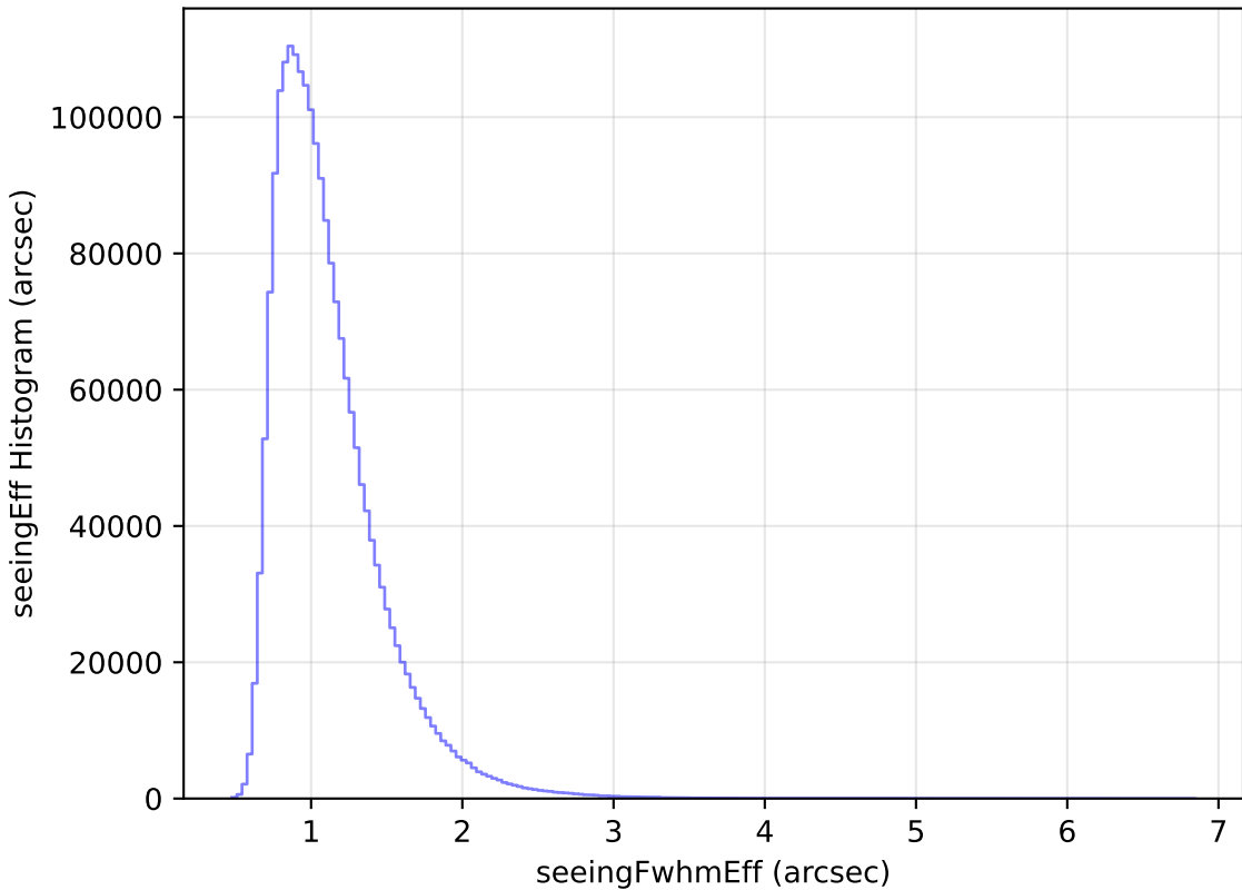
ddf_loaded_fl2_v3.4_10yrs All sky all bands: seeingEff Histogram
