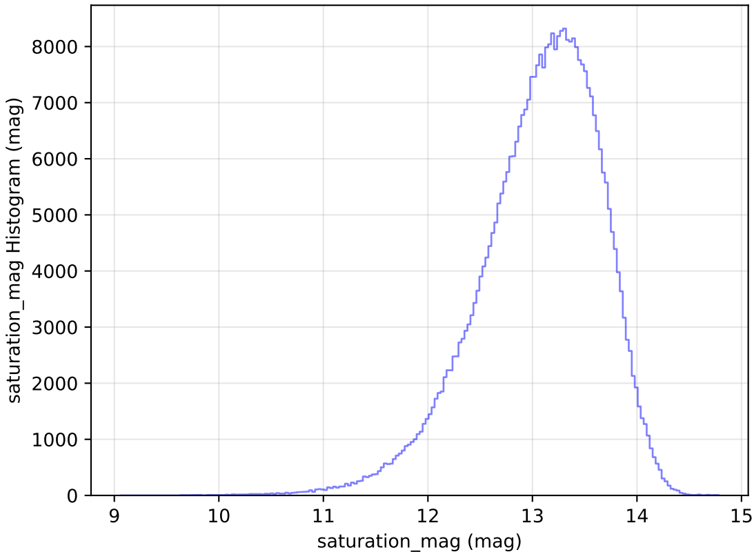
ddf_loaded_fl2_v3.4_10yrs WFD y band: saturation_mag Histogram
