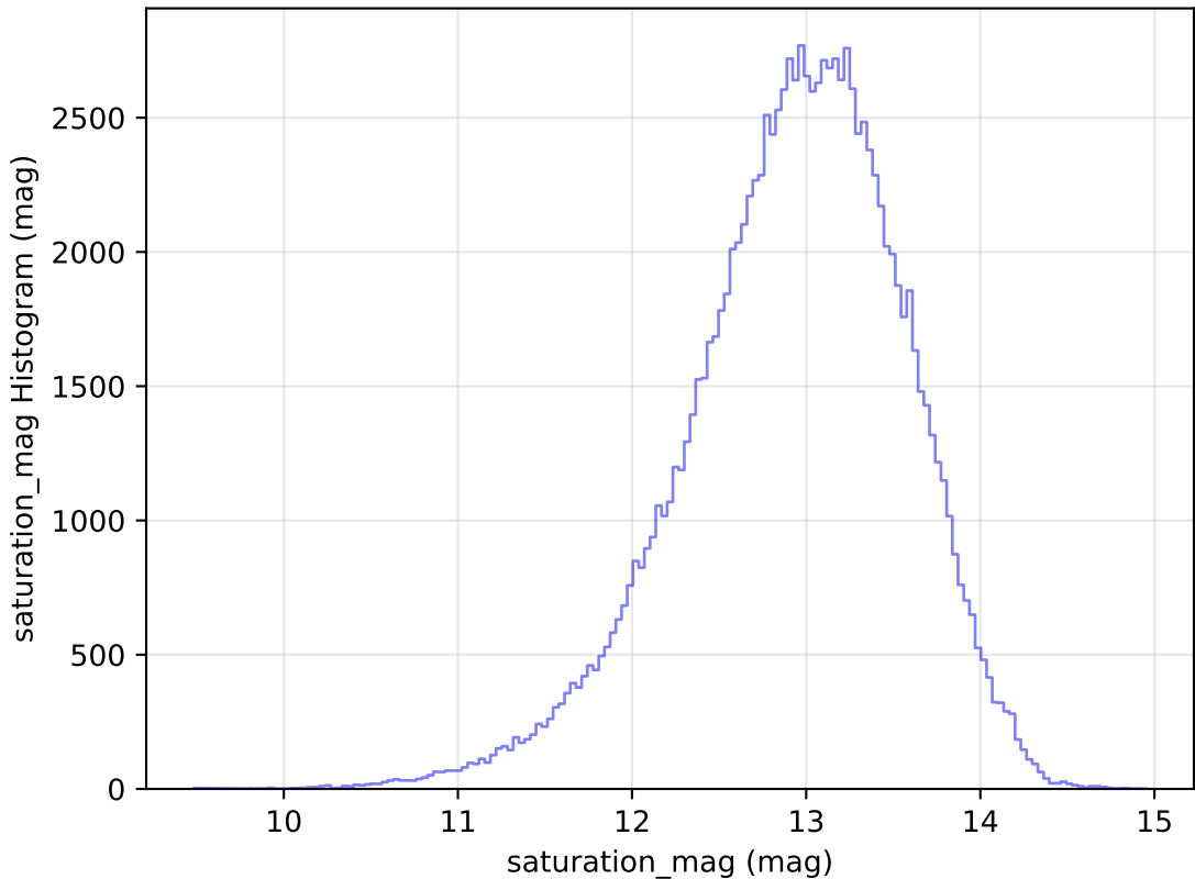
ddf_loaded_fl2_v3.4_10yrs WFD u band: saturation_mag Histogram
