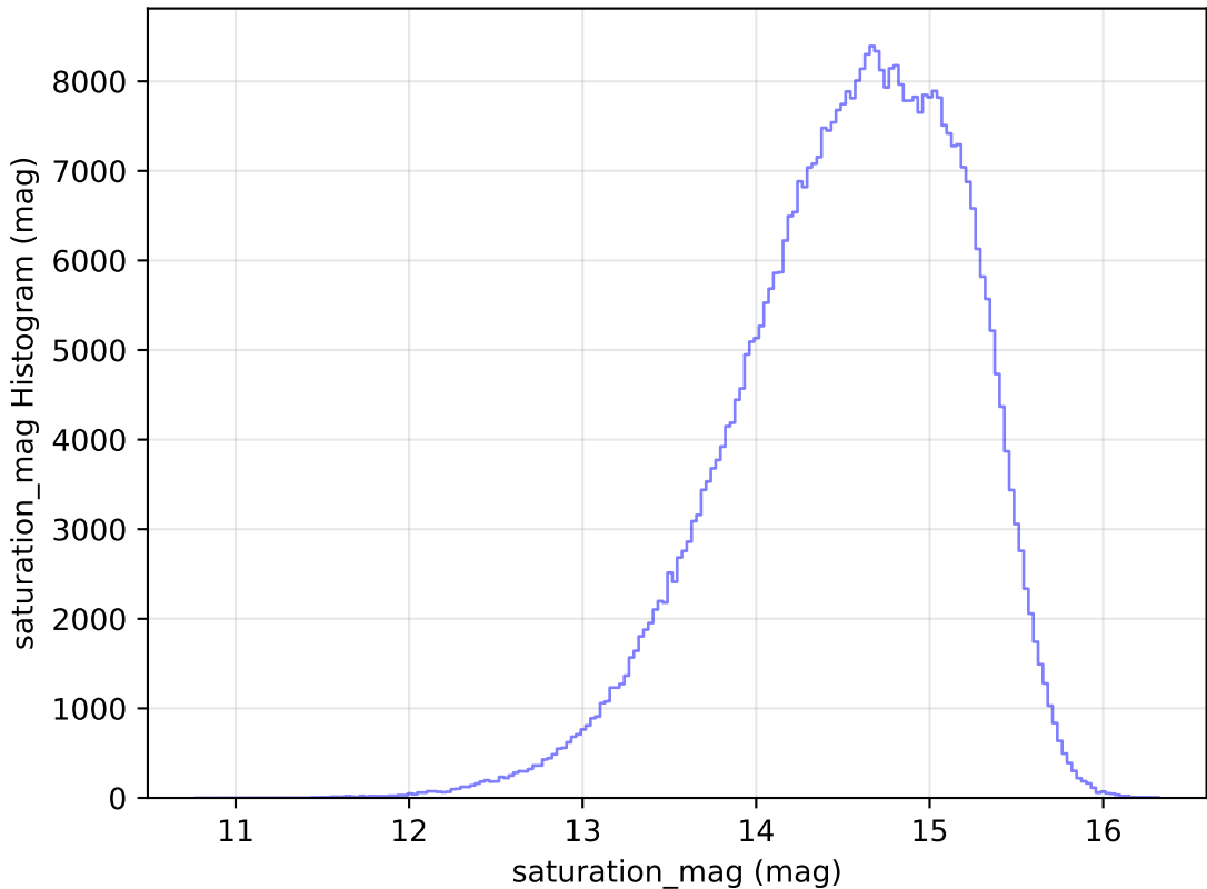
ddf_loaded_fl2_v3.4_10yrs WFD r band: saturation_mag Histogram
