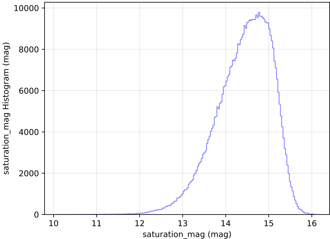
ddf_loaded_fl2_v3.4_10yrs WFD i band: saturation_mag Histogram
