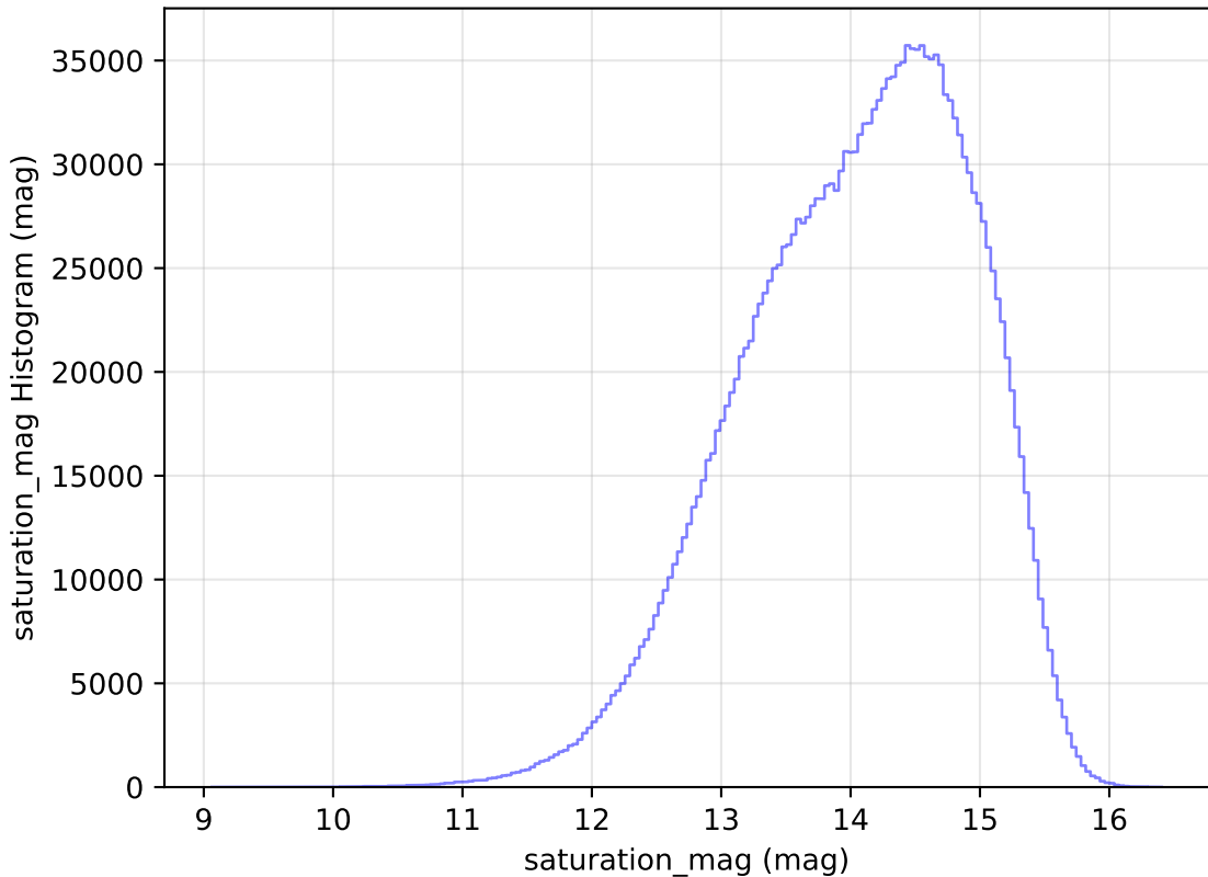
ddf_loaded_fl2_v3.4_10yrs WFD all bands: saturation_mag Histogram
