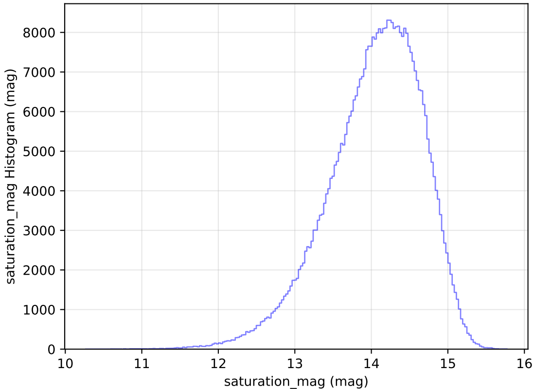
ddf_loaded_fl2_v3.4_10yrs All sky z band: saturation_mag Histogram
