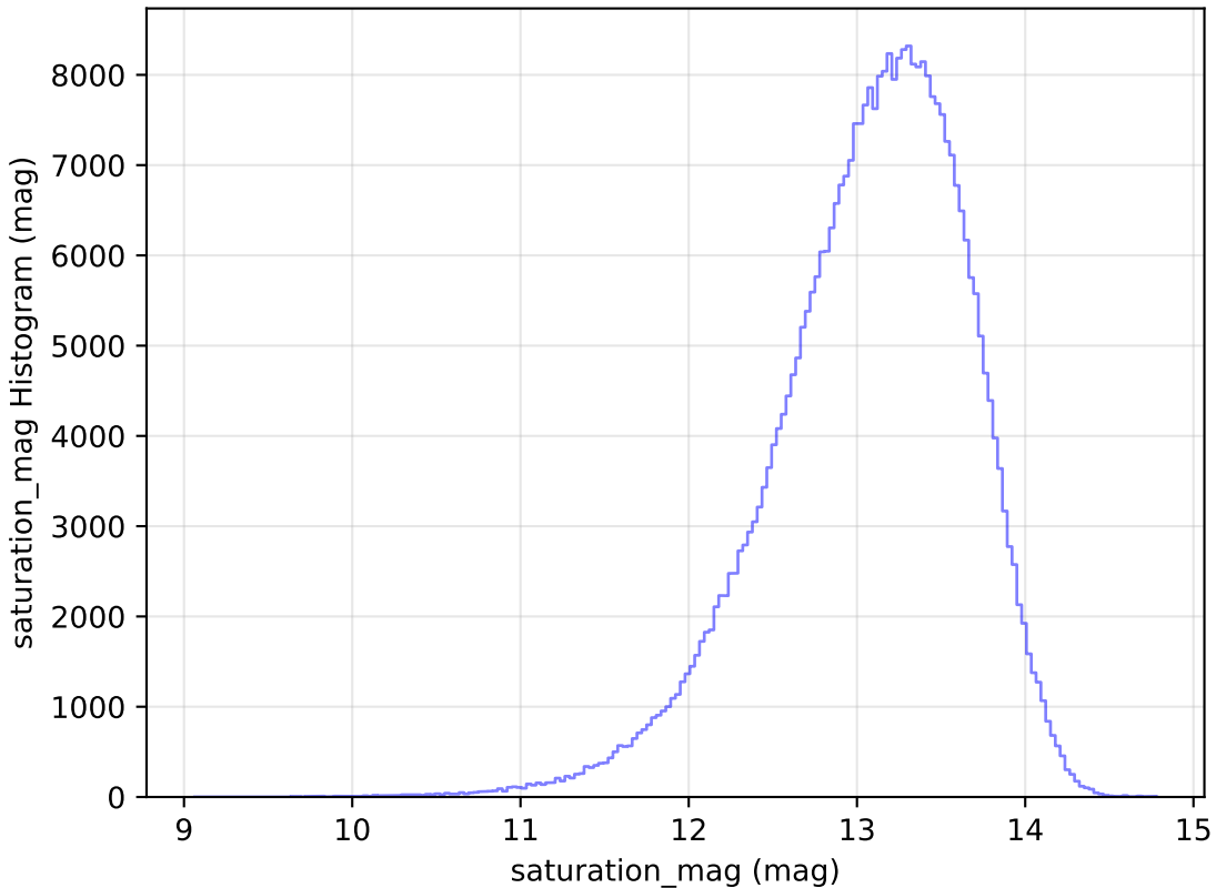
ddf_loaded_fl2_v3.4_10yrs All sky y band: saturation_mag Histogram
