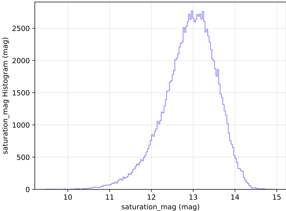
ddf_loaded_fl2_v3.4_10yrs All sky u band: saturation_mag Histogram
