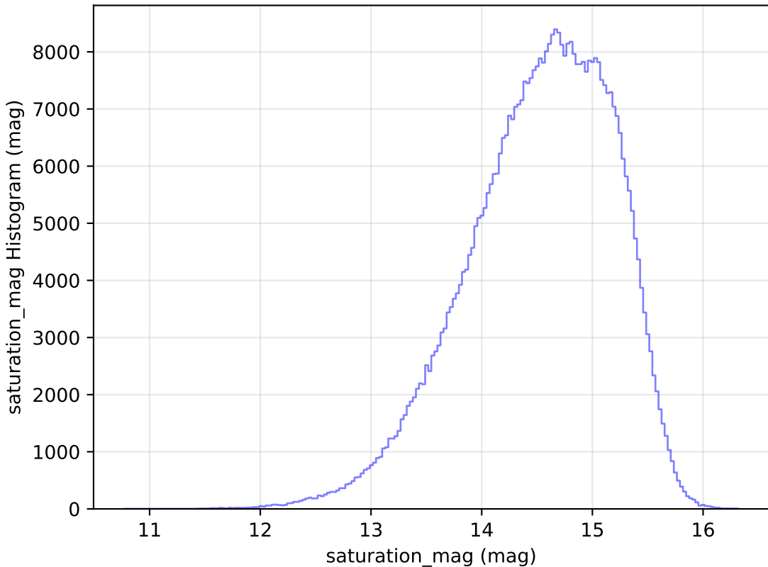
ddf_loaded_fl2_v3.4_10yrs All sky r band: saturation_mag Histogram
