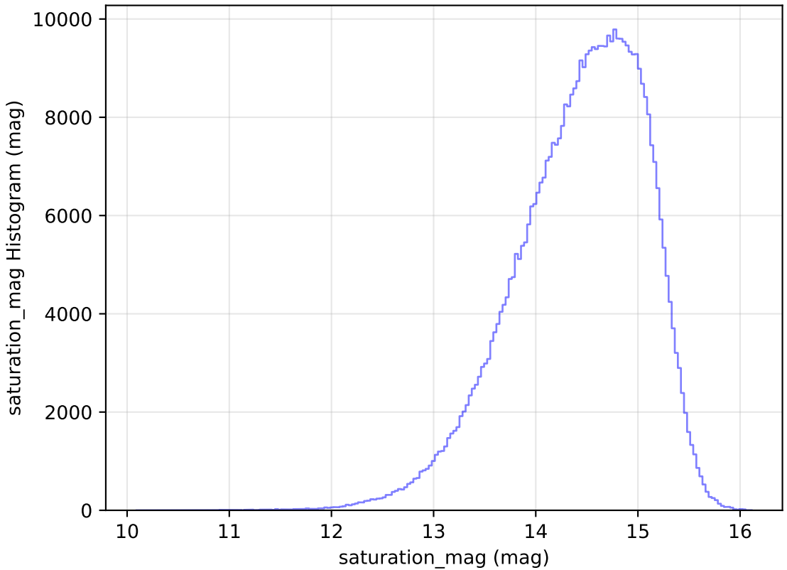
ddf_loaded_fl2_v3.4_10yrs All sky i band: saturation_mag Histogram
