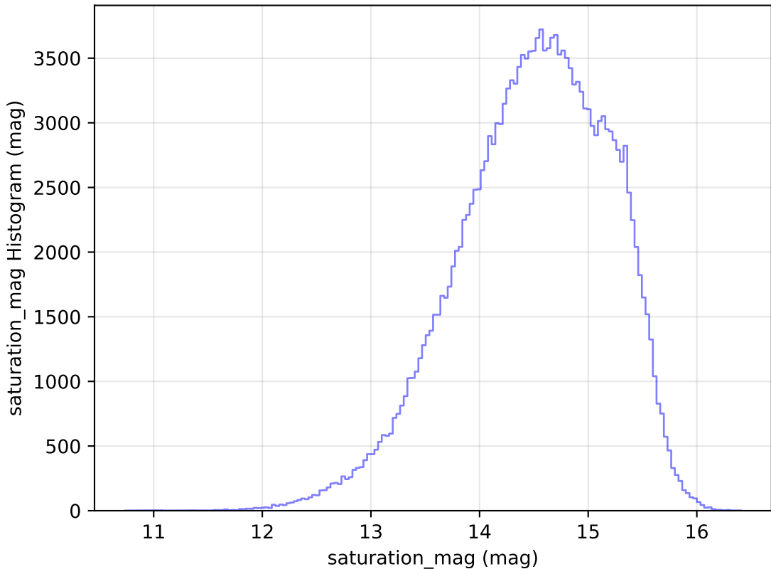
ddf_loaded_fl2_v3.4_10yrs All sky g band: saturation_mag Histogram
