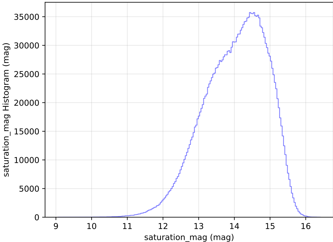
ddf_loaded_fl2_v3.4_10yrs All sky all bands: saturation_mag Histogram
