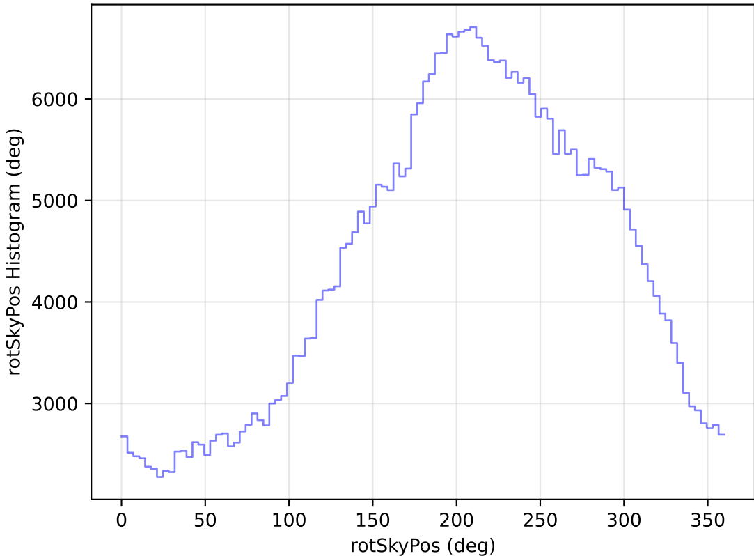
ddf_loaded_fl2_v3.4_10yrs WFD z band: rotSkyPos Histogram
