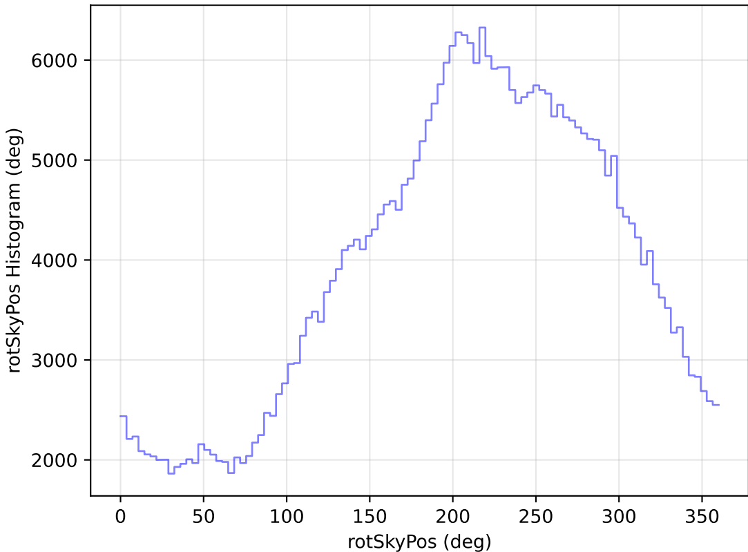
ddf_loaded_fl2_v3.4_10yrs WFD y band: rotSkyPos Histogram
