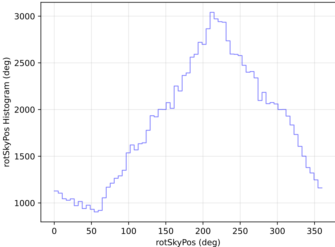
ddf_loaded_fl2_v3.4_10yrs WFD u band: rotSkyPos Histogram
